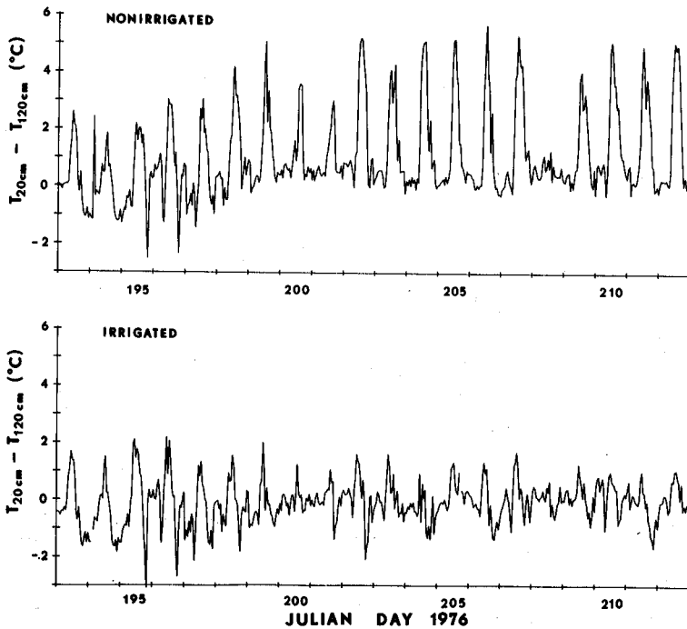
Fig. 4. Soybean canopy air temperature differences between the 20- and 120-cm height in the irrigated and nonirrigated treatments as a function of time.
