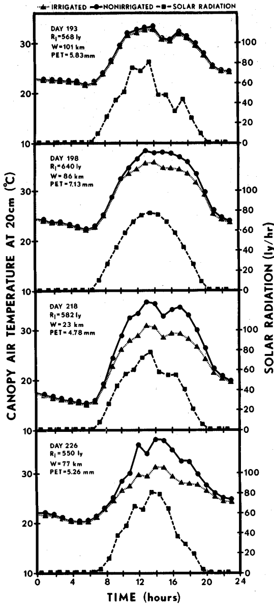
Fig. 3. Within soybean canopy air temperature at the 20-cm height in irrigated and nonirrigated treatments and solar radiation on selected days during the drought. R_i = solar radiation, W = wind run, and PET = potential evapotranspiration — all are daily values.
