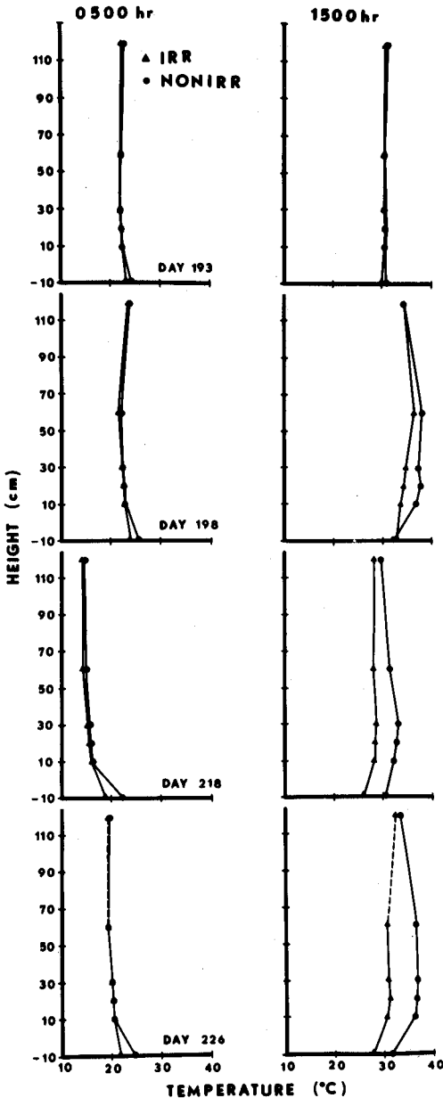
Fig. 5. Air temperature profiles in the soybean canopies near the minimum and maximum temperatures on selected days.
