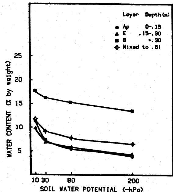
Figure 1. Characteristic curves for three soil layers and lab mix.
