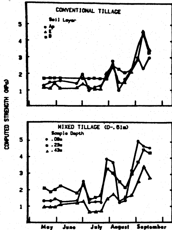
Figure 4. Soil strength computed from regression equation as a function of time for the conventional and deeply mixed tillage treatments.
