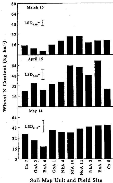
Figure 4. Amount of N in aboveground biomass of wheat at 10 sites for three sampling dates in 1994
