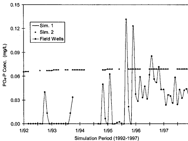
Figure 5. Observed and GLEAMS simulated PO_4-P leachate concentrations during the study period.
