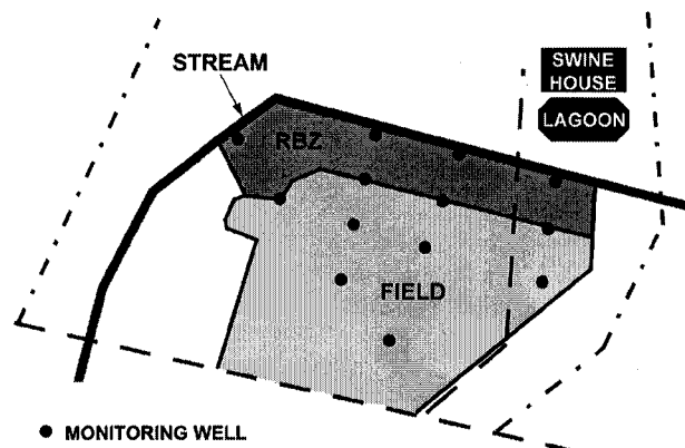
Figure 1. Project site, plan view (not to scale).
