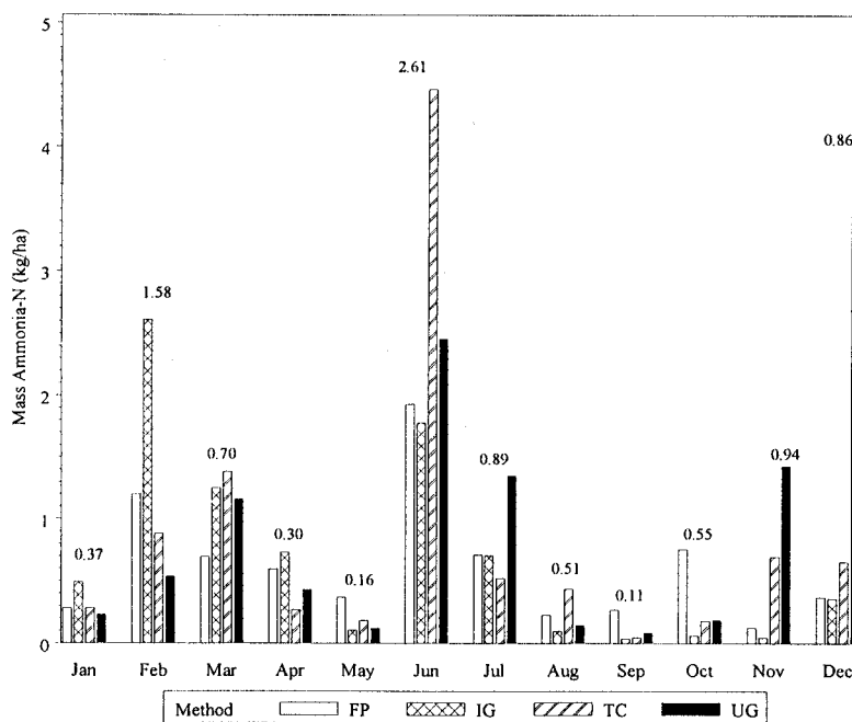
Figure 8. Mean 1995 monthly mass ammonia-N loading for the Herrings Marsh Run Watershed for the four sampling methods (LSD 0.05 values are shown above each month).
