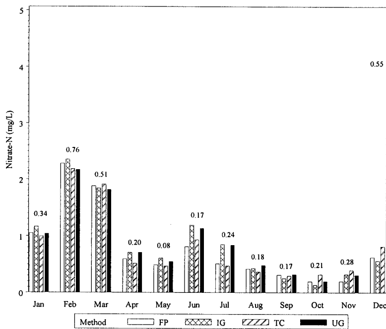
Figure 5. Mean 1995 monthly nitrate-N concentrations for the Herrings Marsh Run Watershed for the four sampling methods (LSD 0.05 values are shown above each month).
