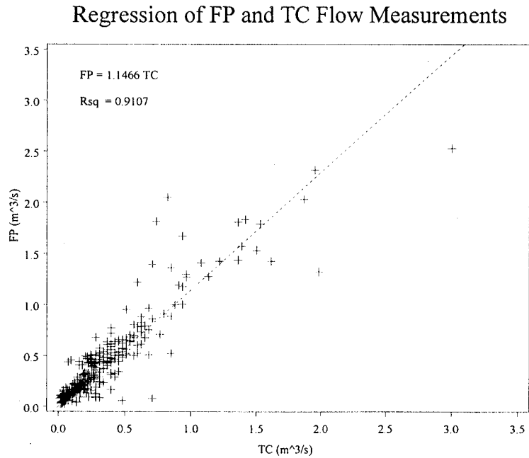
Figure 2. Regression of Flow-Proportional (FP) and Time Compositd (TC) flow measurements.
