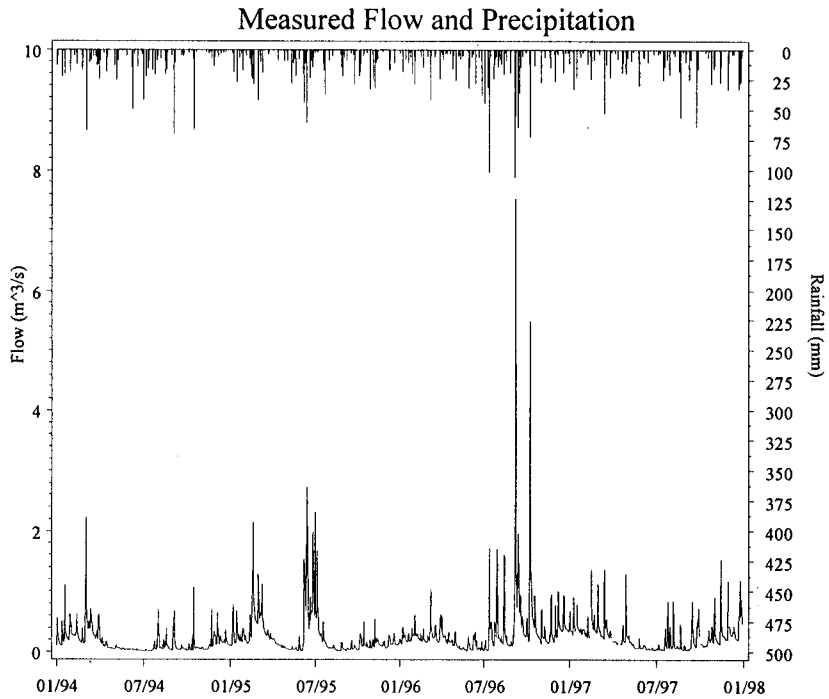
Figure 1. USGS stream flow and rainfall for the Herring Marsh Run Watershed.
