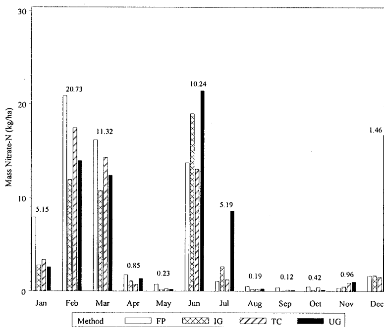
Figure 6. Mean 1995 monthly mass nitrate-N loading for the Herrings Marsh Run Watershed for the four sampling methods (LSD 0.05 values are shown above each month).
