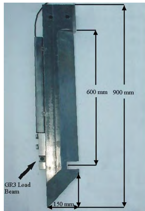
Figure 1. OSSS shank without sensing tips.
