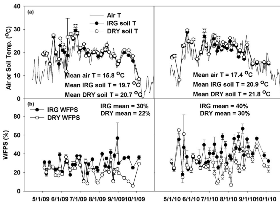
Fig. 2. (a) Air temperature and mean soil temperature, and (b) mean water-filled pore space (WFPS) at the 0.05-m depth at the time of N_2O sampling in fully irrigated (IRG) and minimum-irrigated (DRY) plots during 2009 and 2010. Standard errors are denoted by vertical bars.
