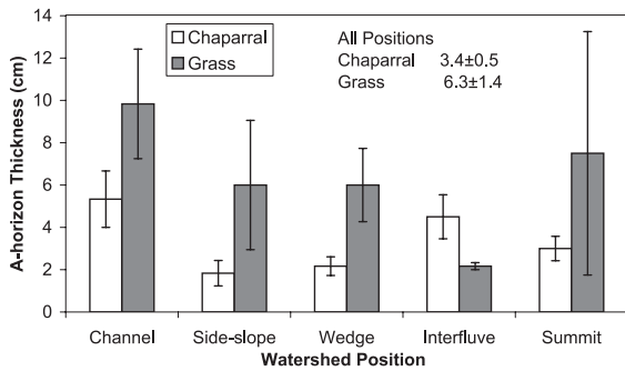
Fig. 5. Mean thickness of the A-horizon at each watershed element for chaparral and grass ( n=3 ). Data are reported with bars to show standard error. Mean A-horizon thickness for each vegetation type is also shown ( n=15 ). The difference between vegetation types has a p=0.06 and an F -test showed that variability is significantly higher ( p<0.001 ) under grass.
