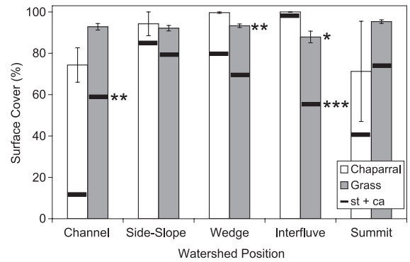
Fig. 3. Total surface cover by watershed element, including stems/tussocks, canopy, litter and mineral material \geq 2 mm diameter. There is significantly more variability in total surface cover under chaparral. The cover provided by only stems/tussocks (st) plus canopy (ca) is shown by the position of the thick black lines. Grass interfluves have significantly less canopy cover than other grass watershed elements or chaparral interfluves. Level of significance of the difference between vegetation types is indicated by *, ** and *** ( p \leq 0.05 , 0.01 and 0.001, respectively). Cover was sampled along 3-m transects within each of the five watershed elements in each of the six watersheds. Data are reported with bars to show standard error.
