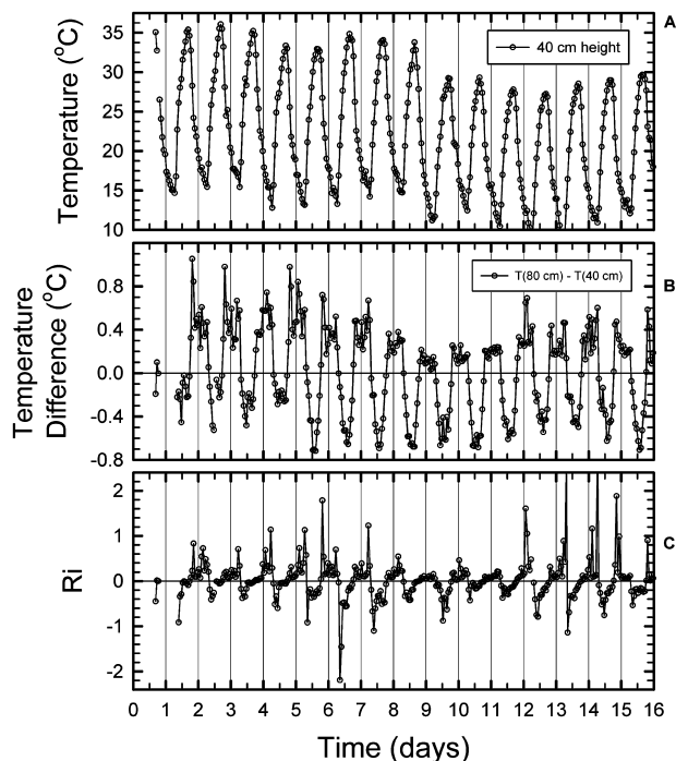
FIGURE 1. Air temperature ( ^{\circ}\text{C} ) at 40 cm height above the soil surface (A), temperature difference between 80 and 40 cm heights (B), and gradient Richardson's number (C). Integer values on the time axis indicate midnight.
