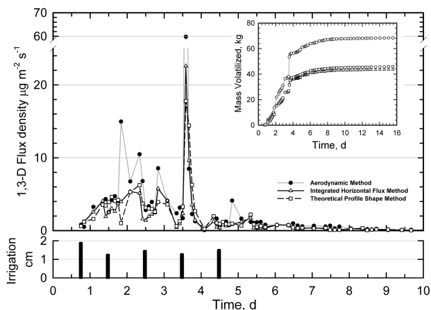
FIGURE 4. Volatilization rate ( \mu\text{g m}^{-2} \text{ s}^{-1} ) and timing and amount of irrigation water as a function of time (d) after application for the aerodynamic (solid line, circles), integrated horizontal flux (solid line, triangles), theoretical profile shape methods (dashed line, squares). The inset shows cumulative 1,3-D emission as a function of time after application.
