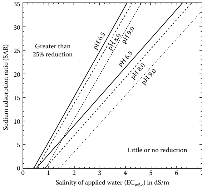
FIGURE 3.2 Sodicity hazard of irrigation water on water infiltration as related to EC, SAR, and pH. (After Suarez, D.L. Irrigation water quality assessments, in Agricultural Salinity Assessment and Management , ed. W. Wallender, Chap. 11, Am. Soc. Civil. Eng. , New York, 2010, in press.)
