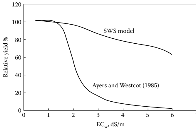
FIGURE 3.3 Comparison of SWS model (Ayers and Westcot, 1985; Suarez et al., 2010) predicted crop relative yield as related to irrigation water EC, for a crop with an h_{50} = -50\text{m} ( -0.5\text{MPa} ), ET_p = 200\text{cm} and 209\text{cm} applied water.
