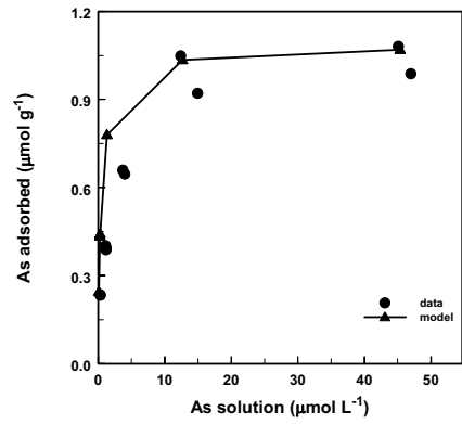
Arsenate adsorption on NE1 25-30 soil
