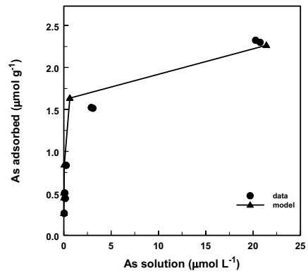
Arsenate adsorption on NE2 16-21 soil
