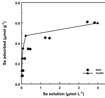
Selenite adsorption on NE2 16-21 soil
