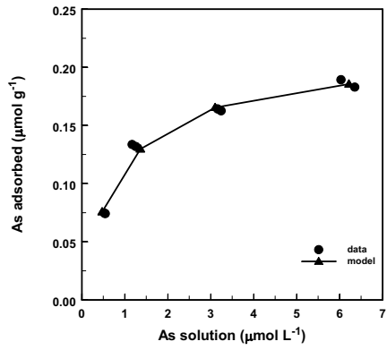
Arsenite adsorption on NE2 16-21 soil
