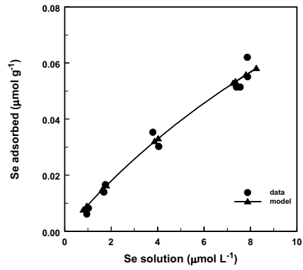
Selenate adsorption on NE2 16-21 soil
