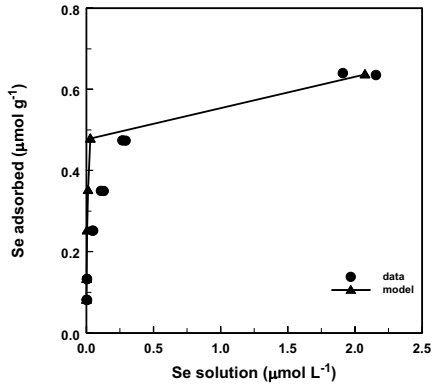
Selenite adsorption on NE3 50-54 soil
