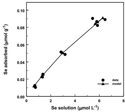
Selenate adsorption on NE3 50-64 soil
