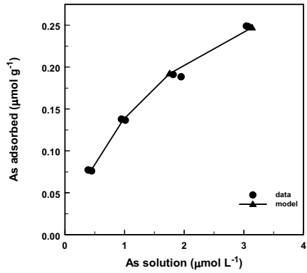
Arsenite adsorption on NE3 50-54 soil
