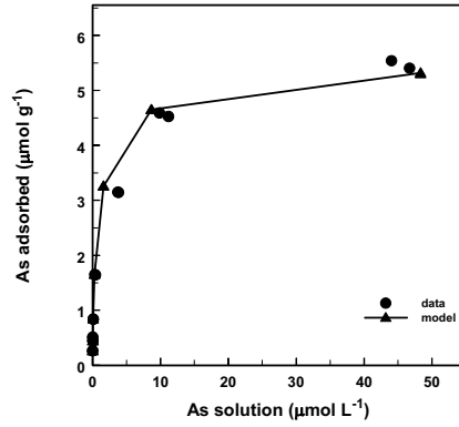
Arsenate adsorption on NE3 50-54 soil
