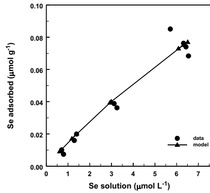
Selenate adsorption on NE4 46-50 soil
