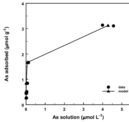
Arsenate adsorption on NE4 46-50 soil
