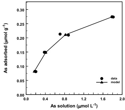
Arsenite adsorption on NE4 46-50 soil
