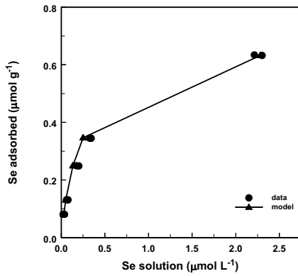
Selenite adsorption on NE4 46-50 soil
