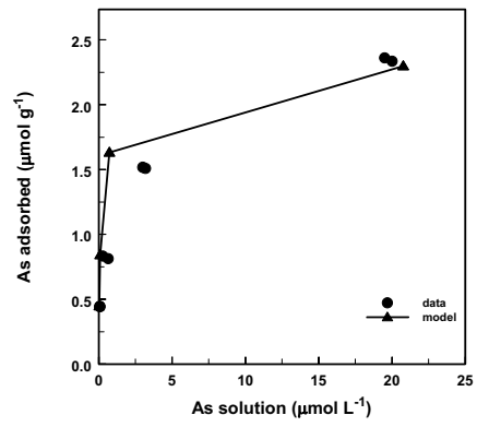
Arsenate adsorption on SE1 48.5 soil
