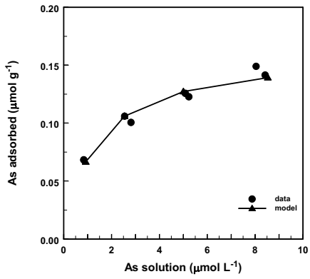
Arsenite adsorption on SE1 48.5 soil
