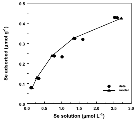
Selenite adsorption on SE1 48.5 soil
