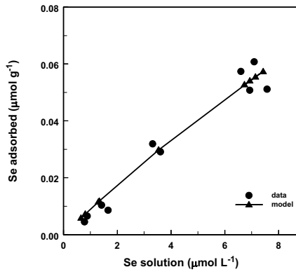
Selenate adsorption on SE1 48.5 soil
