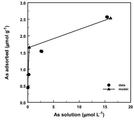
Arsenate adsorption on SE1 60 soil
