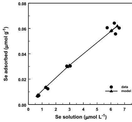
Selenate adsorption on SE1 60 soil
