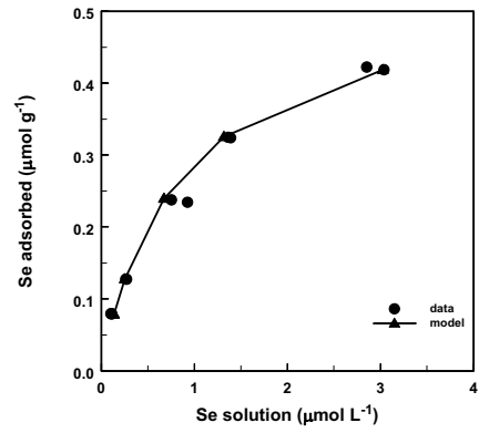
Selenite adsorption on SE1 60 soil
