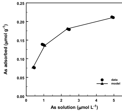
Arsenite adsorption on SE1 60 soil
