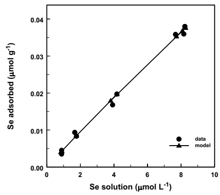
Selenate adsorption on SE2 23.5 soil
