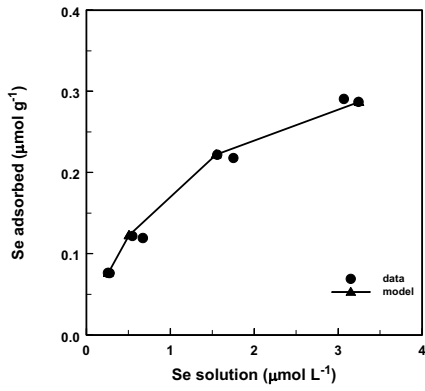
Selenite adsorption on SE2 23.5 soil
