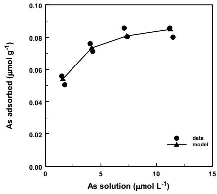
Arsenite adsorption on SE2 23.5 soil
