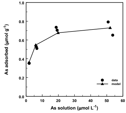
Arsenate adsorption on SE2 23.5 soil
