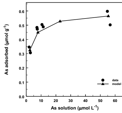
Arsenate adsorption on SE3 38.5 soil
