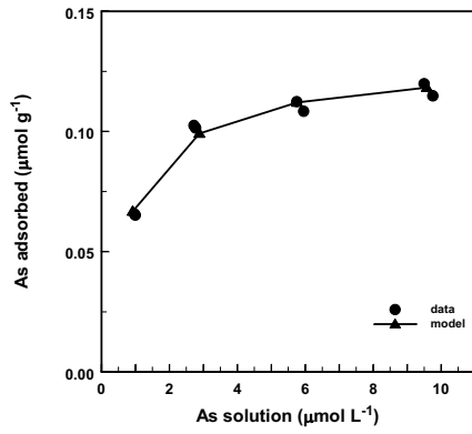
Arsenite adsorption on SE3 38.5 soil
