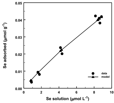
Selenate adsorption on SE3 38.5 soil
