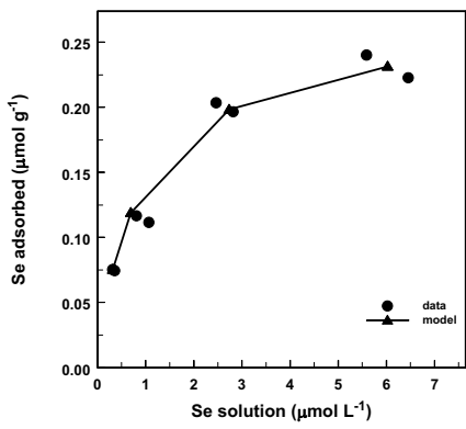
Selenite adsorption on SE3 38.5 soil
