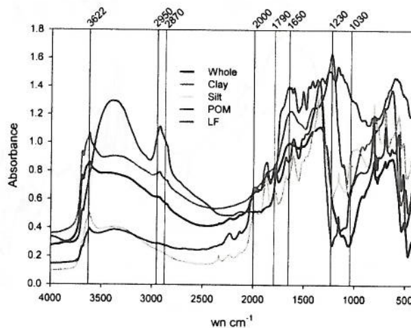
Fig. 1. Mid-infrared spectra of uncultivated whole soil and particle size fractions (0–20 cm depth) from Lamberton, MN. POM, particulate organic matter; LF, light fraction; wn, wavenumbers in \text{cm}^{-1} .
