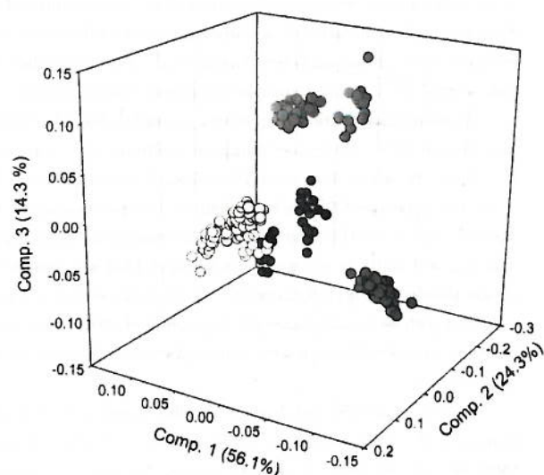
Fig. 3. Principal components analysis of the neat Mid-infrared spectra of uncubated soil and particle size fractions, the 0- to 20-cm depth. All sites together. Light fraction in red, whole soil in black, particulate organic matter in white, silt and clay in green. The percentage of the spectral variance accounted for each component is in parenthesis.
