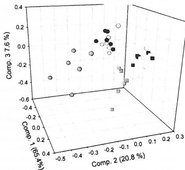
Fig. 8. Principal components analysis of the Lamberton time zero samples. Square samples are decalcified, circles are untreated. Gray are 50+ cm depth, black are 25- to 50-cm depth, and white are the 0- to 20-cm depth. The percentage of the spectral variance accounted for each component is in parenthesis.
