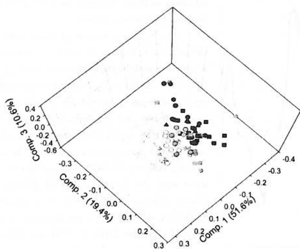
Fig. 9. Principal components analysis of the light fraction samples. All four sites are included. W.K. Kellogg Biological Station samples are squares, Lambertson samples are triangles, Hoytville samples are circles, and Wooster samples are hexagons. Time zero is white, samples incubated for 440 d are gray, and 800-d incubation are black. The percentage of the spectral variance accounted for each component is in parenthesis.
