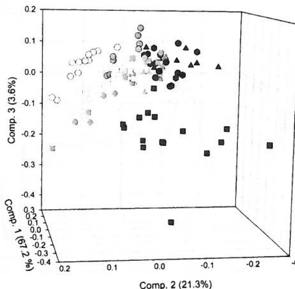
Fig. 10. Principal components analysis of the clay-sized fraction samples. All four sites are included. W.K. Kellogg Biological Station samples are squares, Lambertson samples are triangles, Hoytville samples are circles, and Wooster samples are hexagons. Time zero is white, samples incubated for 440 d are gray, and 800-d incubation are black. The percentage of the spectral variance accounted for each component is in parenthesis
