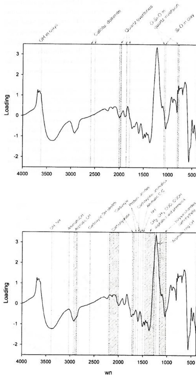
Fig. 6. Component 3 loadings for the principal components analysis of the near mid-infrared spectra of uncubated soil and soil fractions shown in Fig. 3; wn, wavenumbers in cm -1 . Top graph has the mineral bands indicated, bottom graph has the organic bands.
