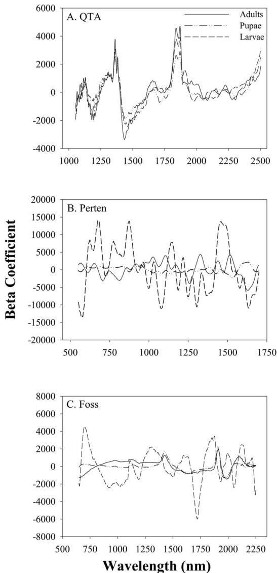
Fig. 5. Beta coefficients showing spectral wavelength bands used by partial least square calibrations to detect insect fragments in wheat flour with three different spectrometers.
