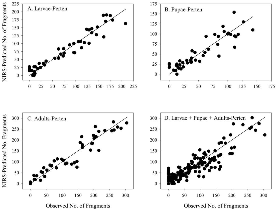
Fig. 3. Relationship between NIRS-predicted and observed number of insect fragments in flour samples produced from wheat infested with larvae (A), pupae (B), premergent adults (C), and the three life stages combined (D). Calibration models generated with the Perten 7000 NIR-instrument. Reference line shows perfect correlation.
