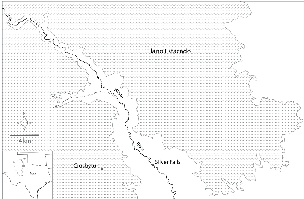
Figure 1. Map of the Llano Estacado showing the location of Silver Falls ( 33.6658^{\circ} N, 101.1589^{\circ} W) in relation to the White River in Blanco Canyon and the small town of Crosbyton, Texas.
