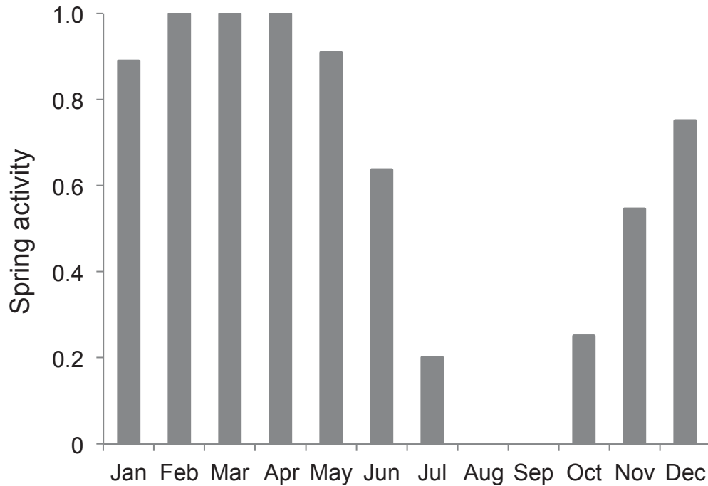
Figure 8. Spring activity based on the fraction of photographs of the White River streambed that provide evidence of a spring-fed baseflow.
