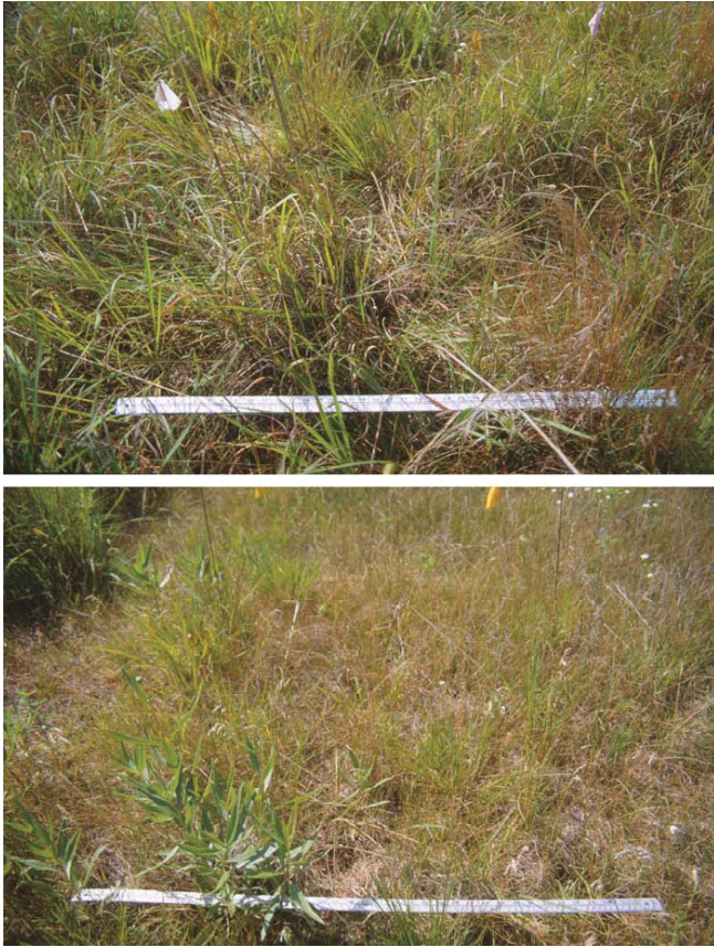
Figure 1. Restored tallgrass prairie dominated by native warm-season grasses (top) produces more biomass and resists weed invasion more effectively than a well-established old-field plant community dominated by introduced cool-season grasses (bottom). Photograph by Dana Blumenthal.
