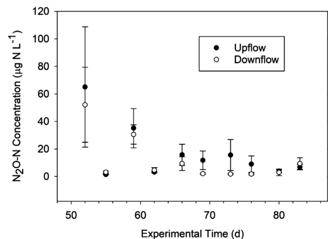
FIGURE 1 Time plot of dissolved N_2O concentration
