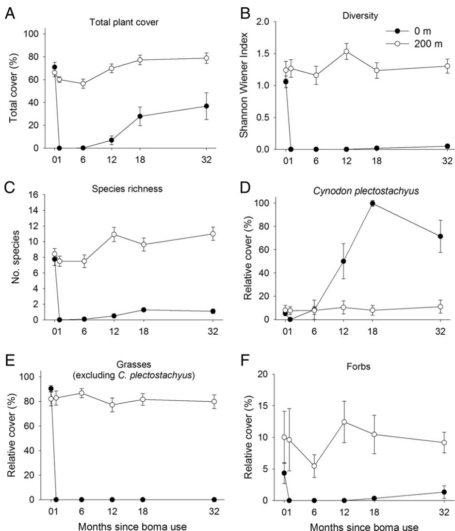
Fig. 3. Herbaceous plant community properties (per 1 m 2 ) inside experimental glades (0 m) vs. reference sites (200 m away) before boma use (0 months) and at 1, 6, 12, 18, and 32 months after abandonment. A, Total plant cover. B, Species diversity. C, Species richness. D, Relative cover of the grass, Cynodon plectostachyus . E, Relative cover of other grasses. F, Relative cover of forbs (note different scale). Means \pm 1 SE.
