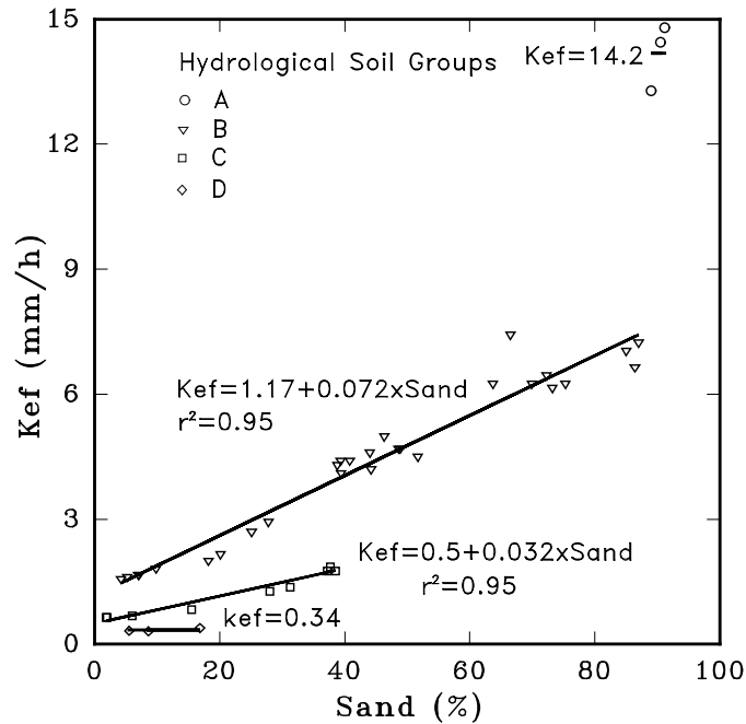
Figure 7.9.6. Optimized effective conductivity values for fallow soil conditions, K_{ef} , plotted versus sand content of the soil. This is for the case of time-invariant conductivity.
