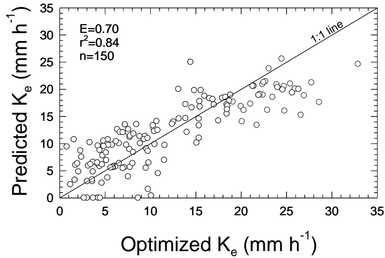
Figure 7.9.7. Comparison of WEPP optimized and predicted effective hydraulic conductivity for rangeland, K_{erange} ( \text{mm}\cdot\text{h}^{-1} ), using Eqs. [7.9.18] and [7.9.19]. E is the Nash-Sutcliffe coefficient of efficiency, r^2 is the coefficient of determination and n is the number of data points.
