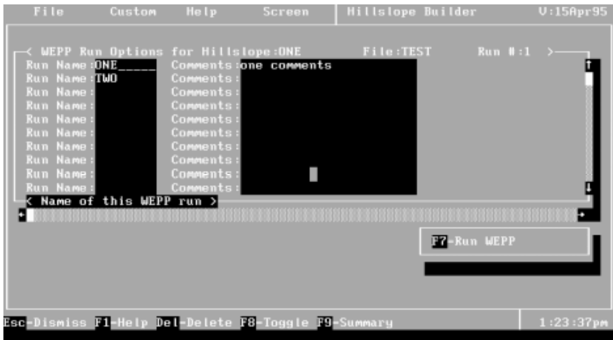
Figure 19. Portion of the WEPP Interface run definition in table mode showing beginning of run definition lines, with sample run name "ONE" entered.
