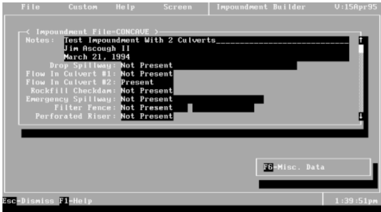
Figure 39. Main screen of the impoundment input file builder.
