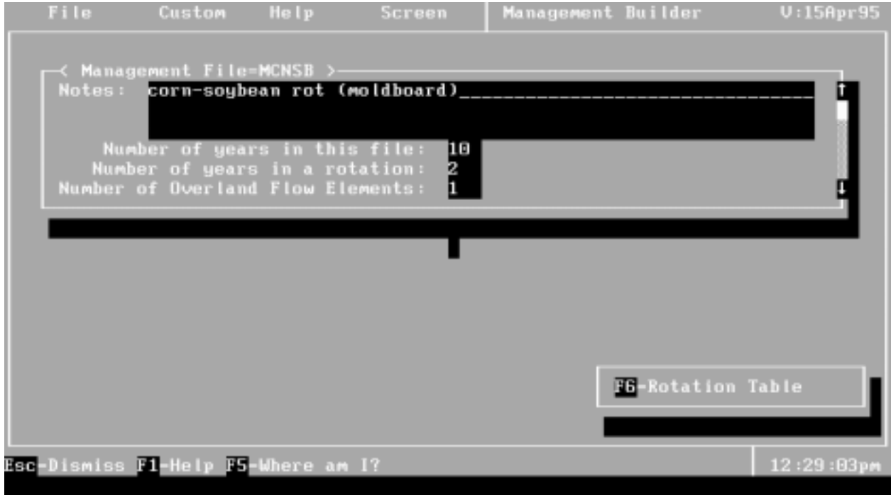
Figure 27. Main Screen of plant/management input file builder.
