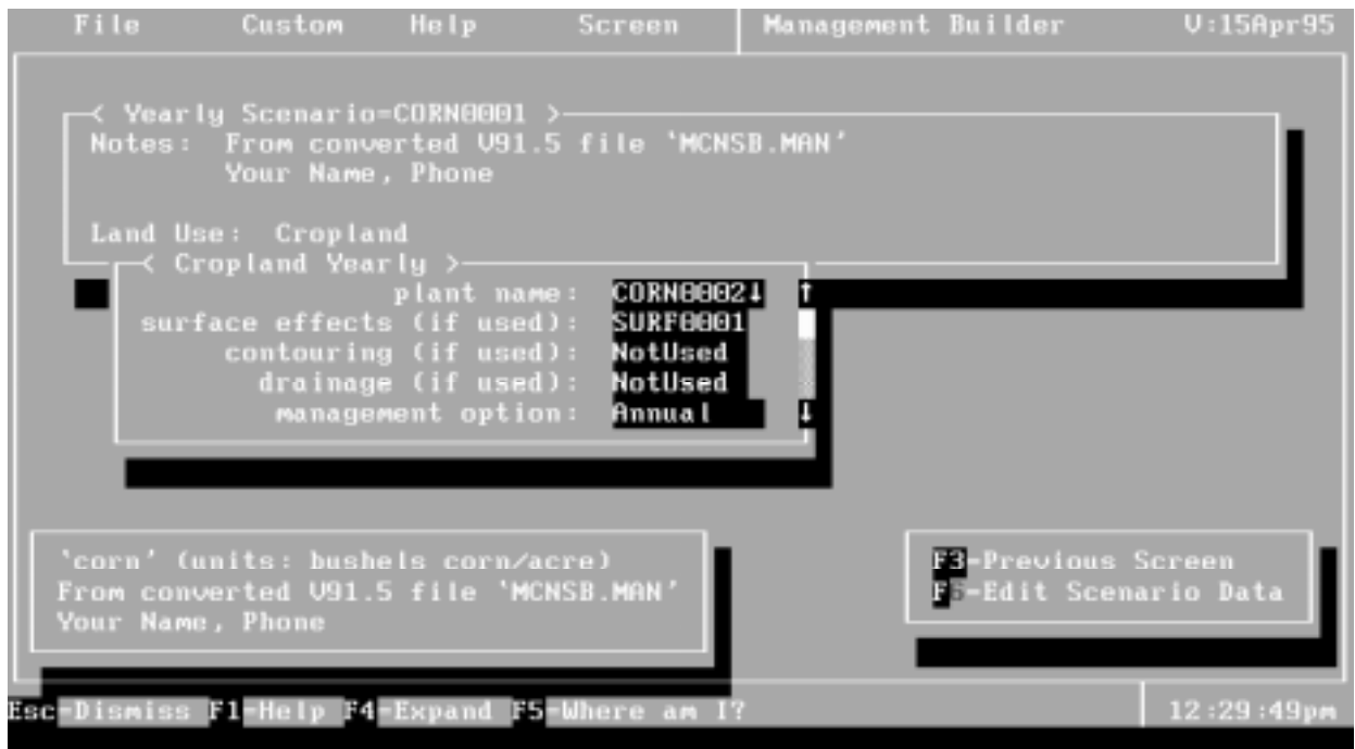
Figure 30. Cropland Yearly edit screen, which is accessed directly below the yearly crop name of the plant/management OFE rotation summary table.
