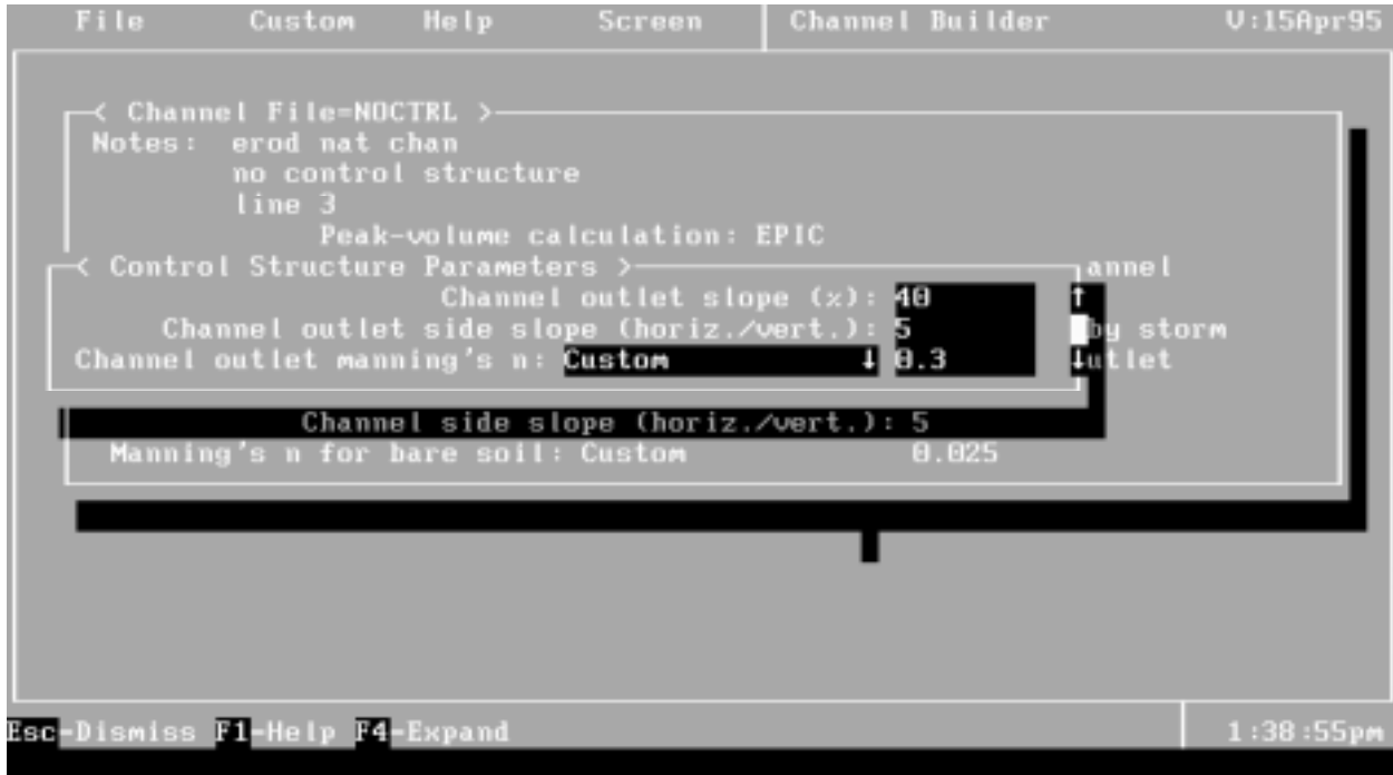
Figure 38. Outlet structure definition screen of the channel input file builder.
