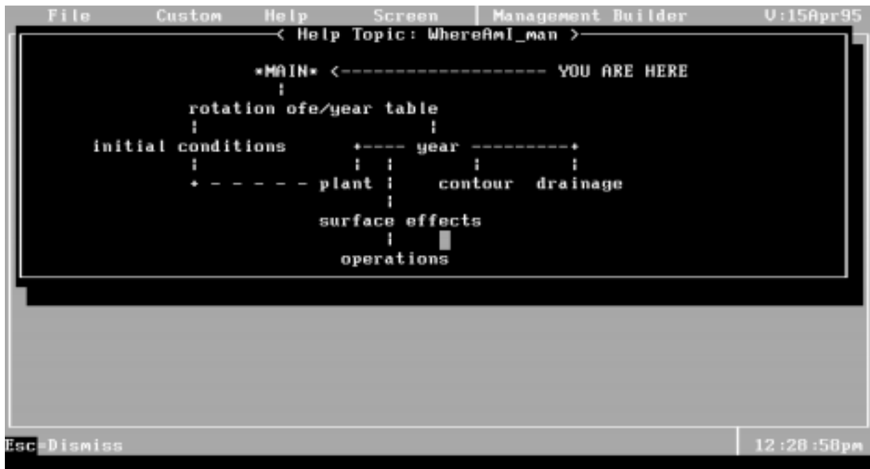
Figure 26. "Where am I" feature of the plant/management input file builder shows the user his/her current location as well as illustrates the builder structure.
