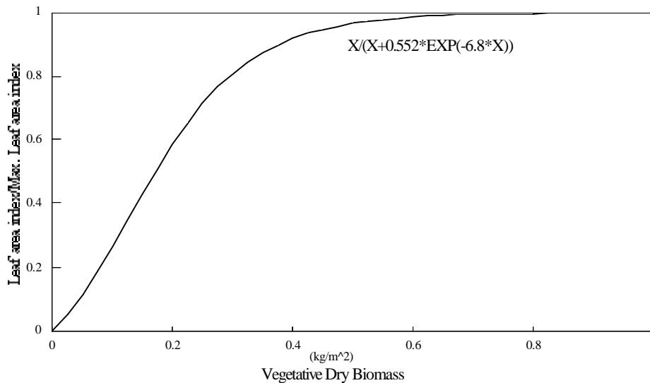
Figure 8. WEPP leaf area and vegetative biomass relationship.
