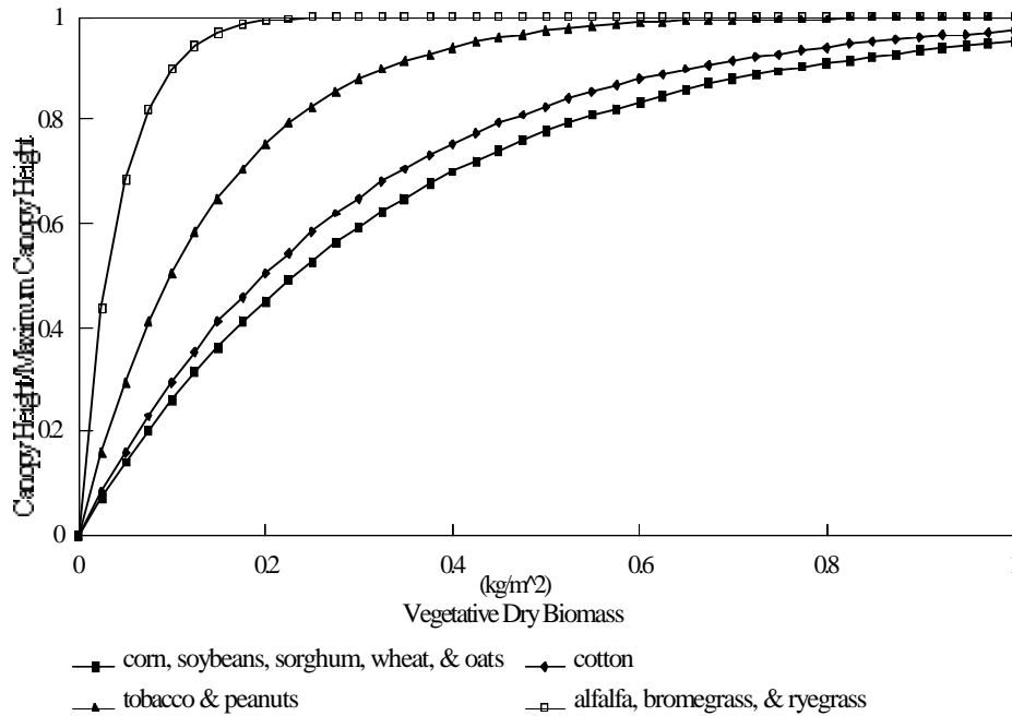
Figure 4. Canopy Height and Biomass Relationship.
