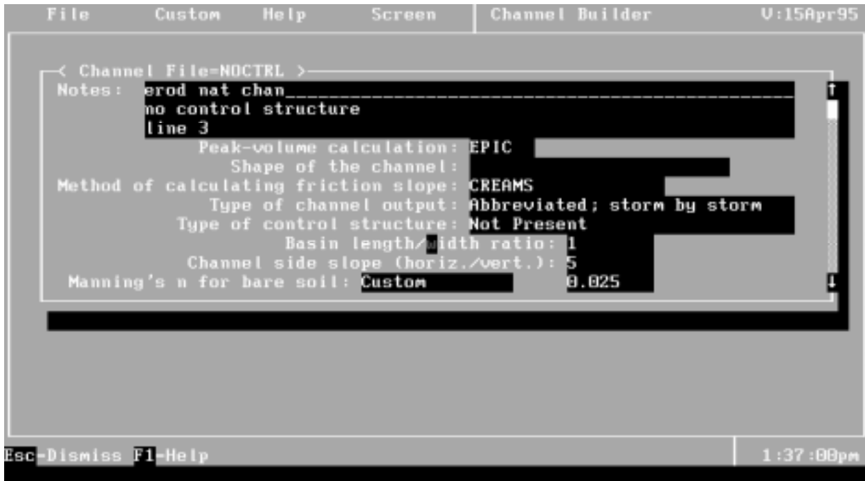
Figure 37. Top portion of the main screen of the channel input builder.
