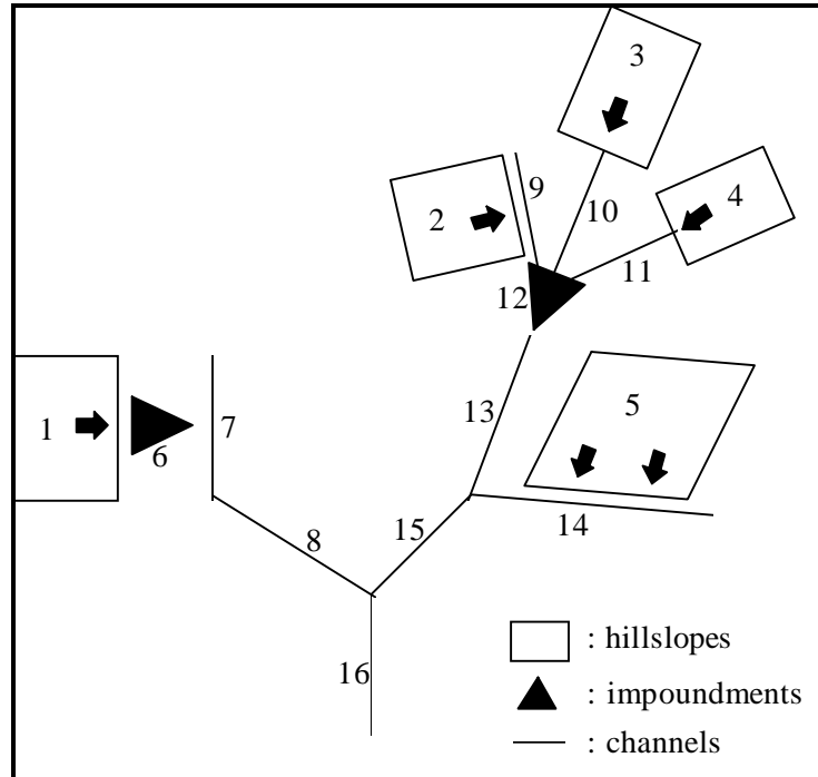
Figure 9. Example of a typical watershed
