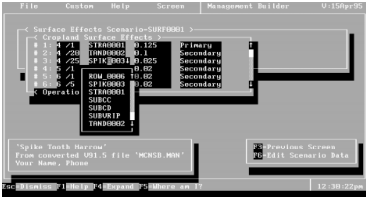
Figure 31. Surface Effects Scenario subscreen of the Plant/Management file builder.
