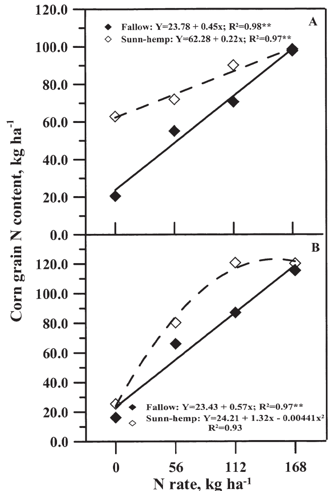
Fig. 2. Corn grain N contents following sunn-hemp and fallow plots measured across four N rates at the E.V. Smith Research and Extension Center in Shorter, AL, for (A) 1991 and (B) 1992.
