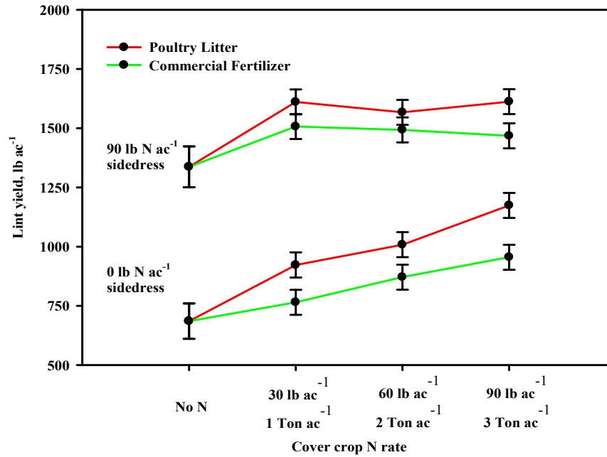
Figure 4. Cotton lint yields measured across two sources of N (commercial fertilizer and poultry litter) applied to the cover crop and two cotton sidedress N rates (0 and 90 lb N ac -1 ) during the 2007 growing season at the Wiregrass Research and Extension Center in Headland, AL.
