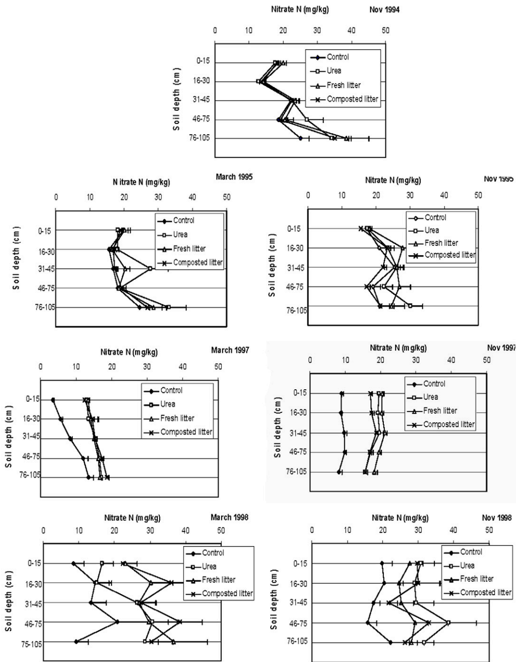
Fig. 6. Nitrate N concentration in soil at different depths as affected by N sources calculated across N rates and nitrification inhibitor, from November 1994 through November 1998, Belle Mina, AL (vertical bars = SE).
