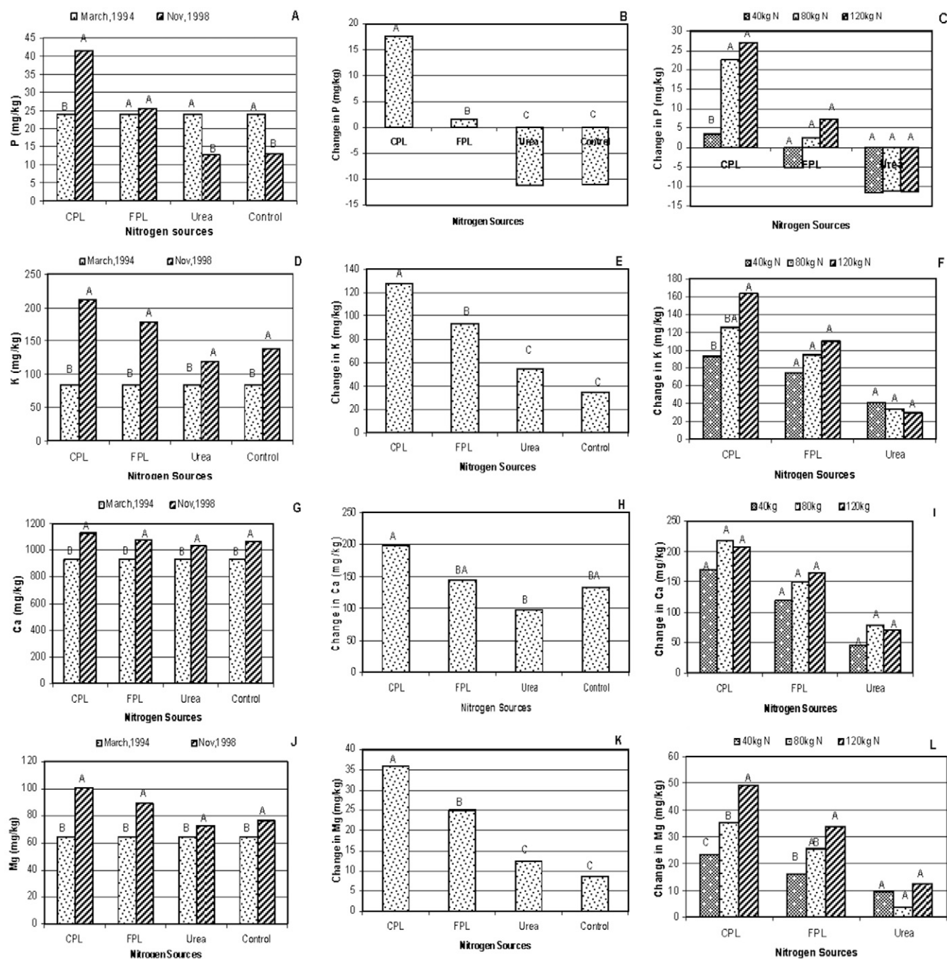
Fig. 7. Influence of N sources on soil P, K, Ca, and Mg concentrations in March 1994 and November 1998 and change in soil P, K, Ca, and Mg due to sources and rates of N. Means under each N source followed by same uppercase letter are not significantly different from each other at P \leq 0.05 . (CPL, composted poultry litter; FPL, fresh poultry litter). Values for graphs A, B, D, E, G, H, J, and K were averaged across N rates and nitrification inhibitor treatments; values for graphs C, F, I, and L were averaged across nitrification inhibitor treatment.
