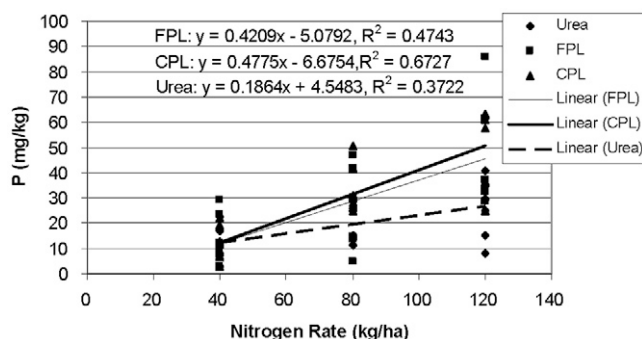
Fig. 8. Soil P concentrations as influenced by sources of N regressed on N equivalent litter application rates in 1998.
