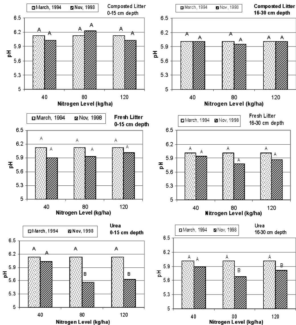
Fig. 2. Soil pH at 0 to 15 and 16 to 30 cm depth in March 1994 and November 1998 as influenced by poultry litter and urea application at different N levels calculated across nitrification inhibitor treatment. Means under each level of N followed by different uppercase letter are significantly different from each other at P \leq 0.05 .
