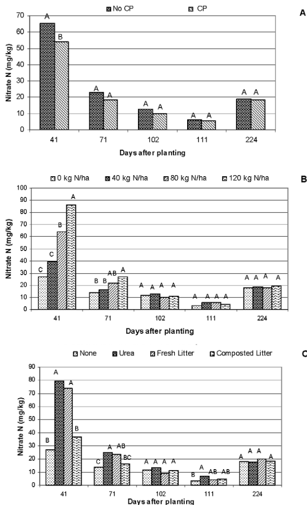
Fig. 3. Effect of CP, N source and rates on surface soil (0–15 cm) nitrate N dynamics during 1994 cotton growing season, Belle Mina, AL. (Means were calculated across the treatments).
