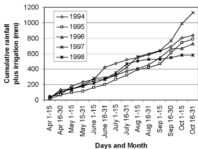
Fig. 1. Cumulative rainfall plus irrigation water applied to cotton from April through October from 1994 through 1998 at Belle Mina, AL.
