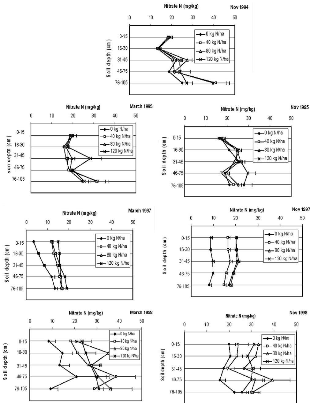
Fig. 5. Nitrate N concentration in soil at different depths as affected by N rates calculated across N sources and nitrification inhibitor from November 1994 through November 1998, Belle Mina, AL (vertical bars = SE).
