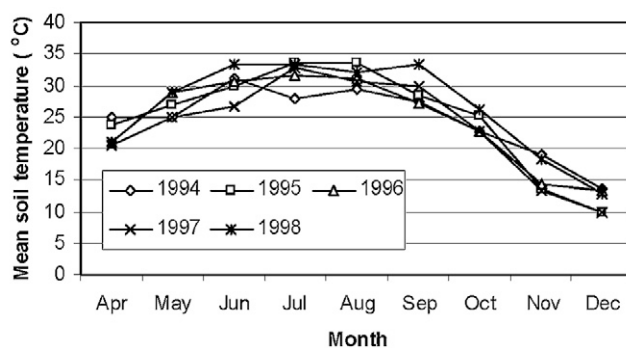
Fig. 4. Mean surface soil temperature from April through December, 1994 to 1998 at Belle Mina, AL.
