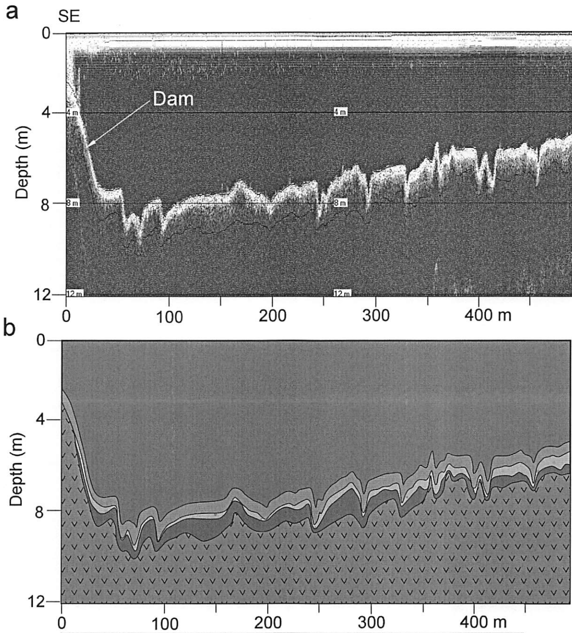
Figure 4-7. Southeast end of White Mound Lake axial profile, Line 50 (see Figure 4-6 for line location). Three acoustic intervals are seen within the sub-bottom in White Mound Lake. All three onlap onto the dam face. Hence, all three must be part of the post-impoundment sediment fill package.
