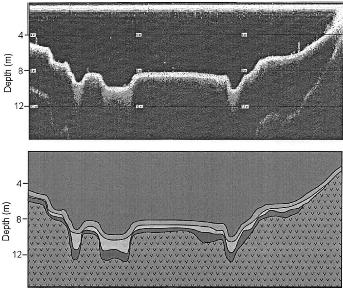
Figure 4-3. Processed Line 11 with interpretation (see Figure 4-1 for line location). The multifrequency acoustic profiles show three distinct sediment layers within the post-impoundment fill.
