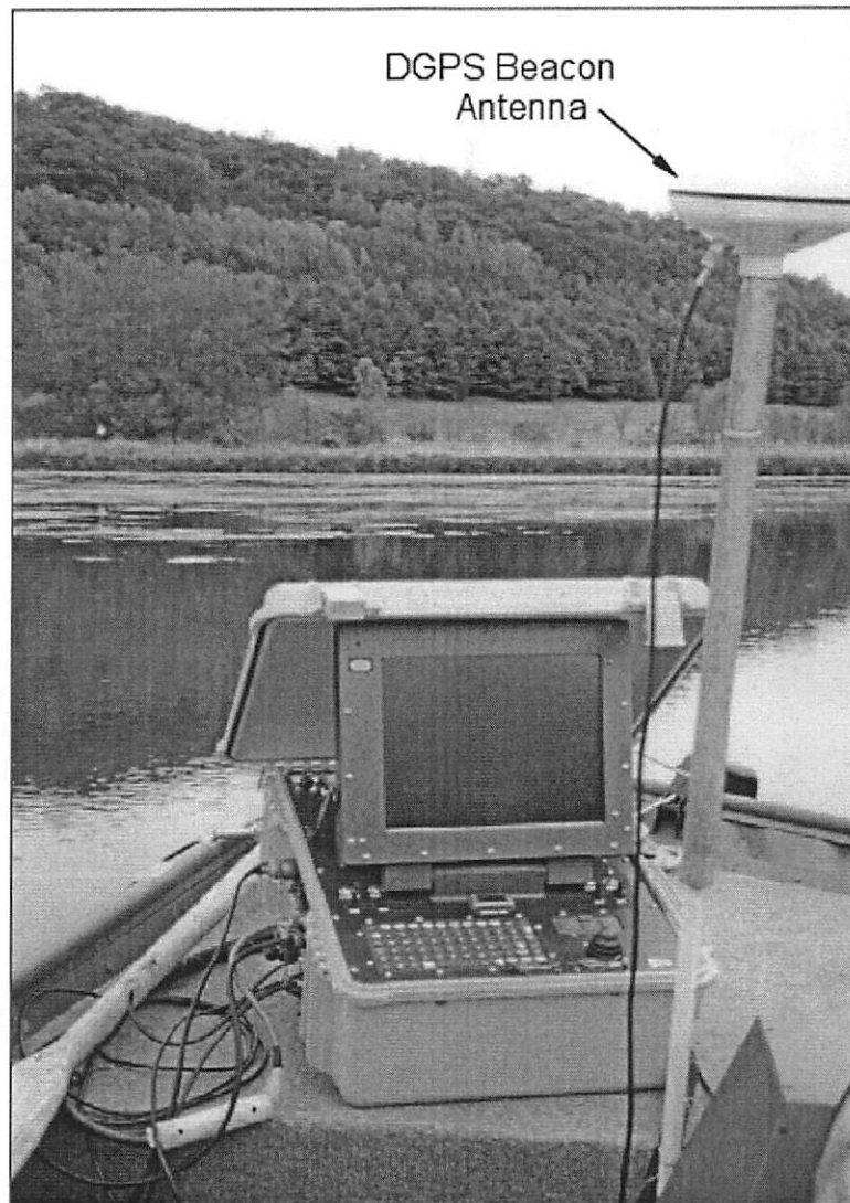
Figure 3-1. Photograph of acoustic profiler control module. All acoustic profiling and DGPS navigation electronics are contained in a compact, water-resistant control module.
