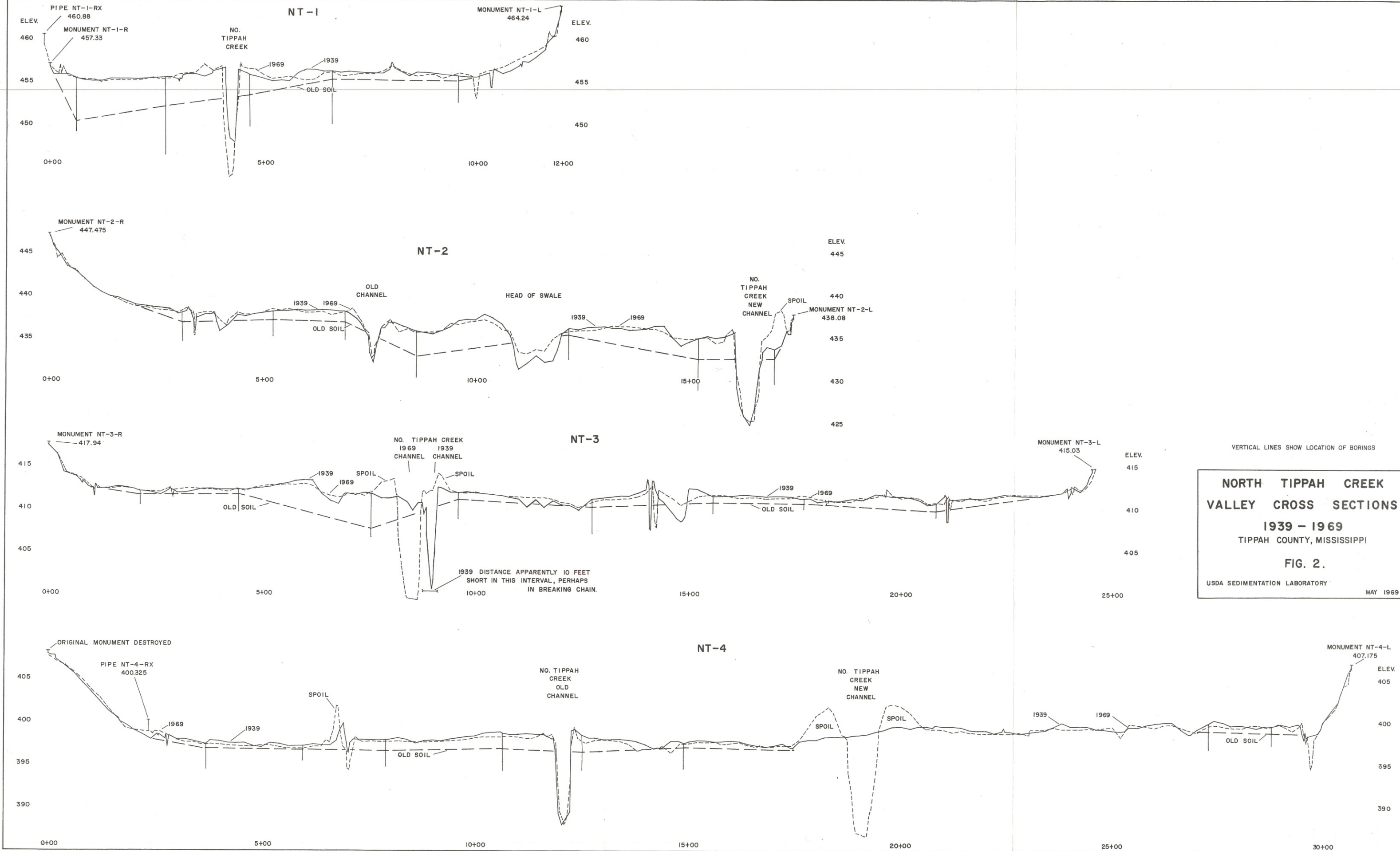
FIG. 2. NORTH TIPPDAH CREEK VALLEY CROSS SECTIONS.
