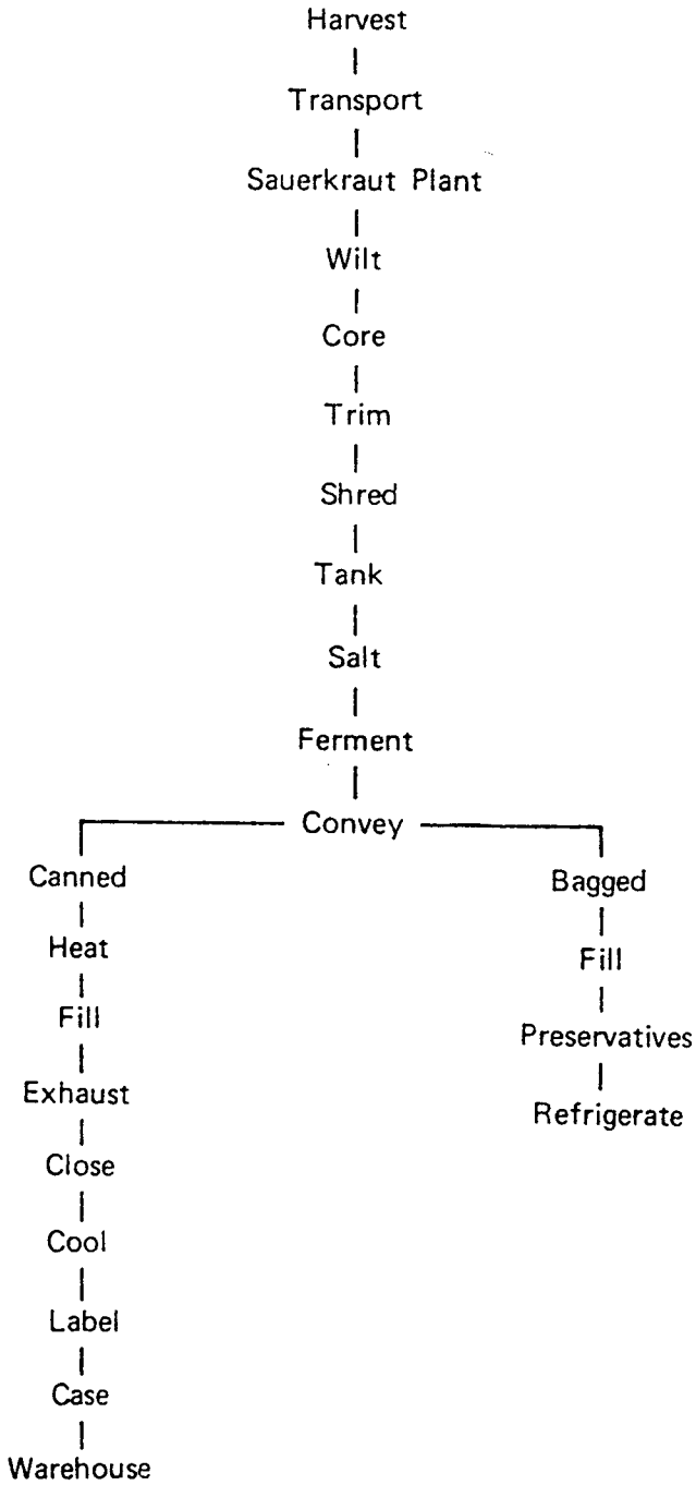
Flow Sheet 6. Flow diagram for sauerkraut processing.
