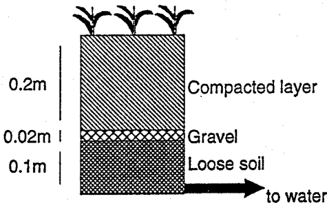
Fig. 1. Experimental set-up.
