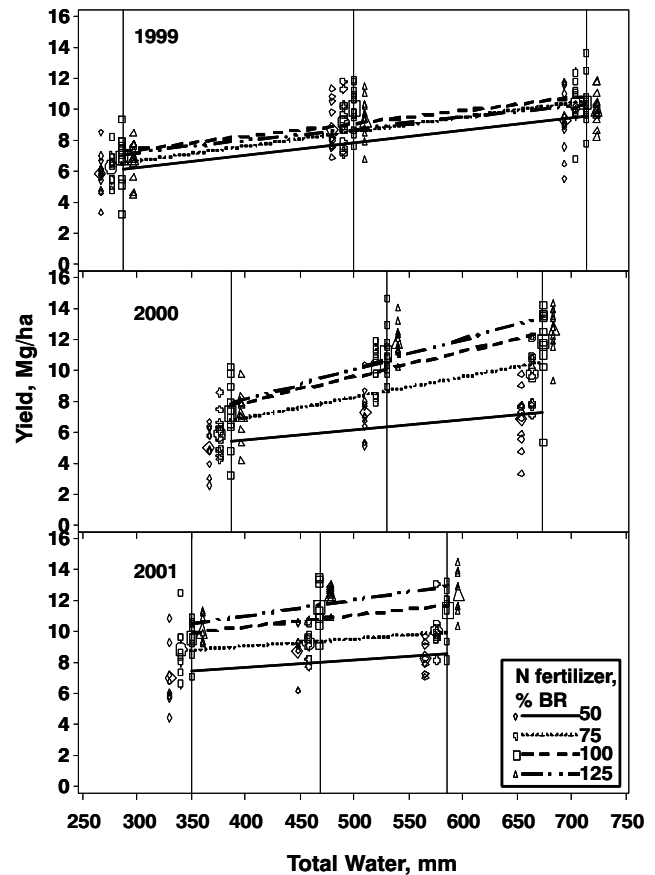
Figure 5. Corn grain yield response to irrigation by N-fertilizer treatment for 1999-2001. Large symbols indicate the mean value for that treatment. Some symbols are offset slightly in horizontal direction to make symbols visible. Vertical lines (from left to right) represent the rainfall, 75%, and 150% irrigation base rates (IBR).
