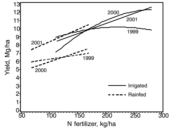
Figure 7. Mean corn grain yield response to N-fertilizer rate for irrigated and rainfed treatments during 1999-2001.
