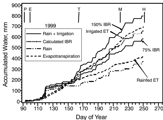
Figure 2. Cumulative rainfall, calculated rainfed and well-watered corn evapotranspiration, and rain plus irrigation for all irrigated treatments during the 1999 corn growing season. The annotations P, E, T, M, and H identify planting, emergence, tasseling, maturity, and harvest dates, respectively, and IBR is irrigation base rate.
