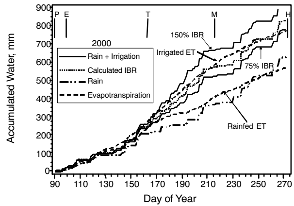
Figure 3. Cumulative rainfall, calculated rainfed and well-watered corn evapotranspiration, and rain plus irrigation for all irrigated treatments during the 2000 corn growing season. The annotations P, E, T, M, and H identify planting, emergence, tasseling, maturity, and harvest dates, respectively, and IBR is irrigation base rate.
