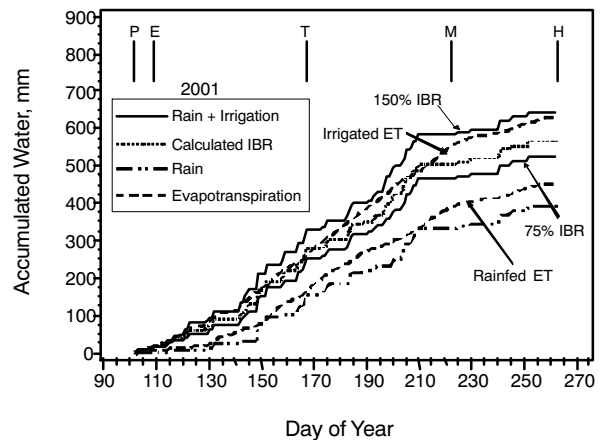
Figure 4. Cumulative rainfall, calculated rainfed and well-watered corn evapotranspiration, and rain plus irrigation for all irrigated treatments during the 2001 corn growing season. The annotations P, E, T, M, and H identify planting, emergence, tasseling, maturity, and harvest dates, respectively, and IBR is irrigation base rate.
