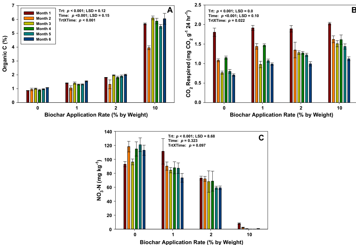
Fig. 2. The effect of increasing biochar application rate and time since application on soil (A) organic C, (B) respired CO 2 , and (C) NO 3 -N. Error bars represent one standard error of the mean (n = 4). LSD = Fisher's Protected Least Significant Difference.
