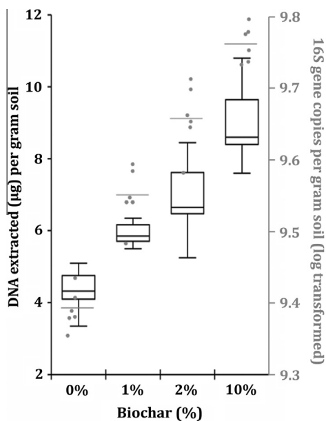
Fig. 3. Box and whisker plot showing concentration (µg) of extracted DNA/g -1 soil (primary Y axis), and dot plot showing 16S rRNA gene copies/g -1 soil (secondary Y axis) for each biochar amendment. All treatments are statistically significant (P < 0.001). Mean lines were calculated for DNA concentrations (n = 12) and 16S rRNA gene copies (n = 144). For 16S rRNA gene copies, each dot represents an averaged value for one month of the study (n = 24).
