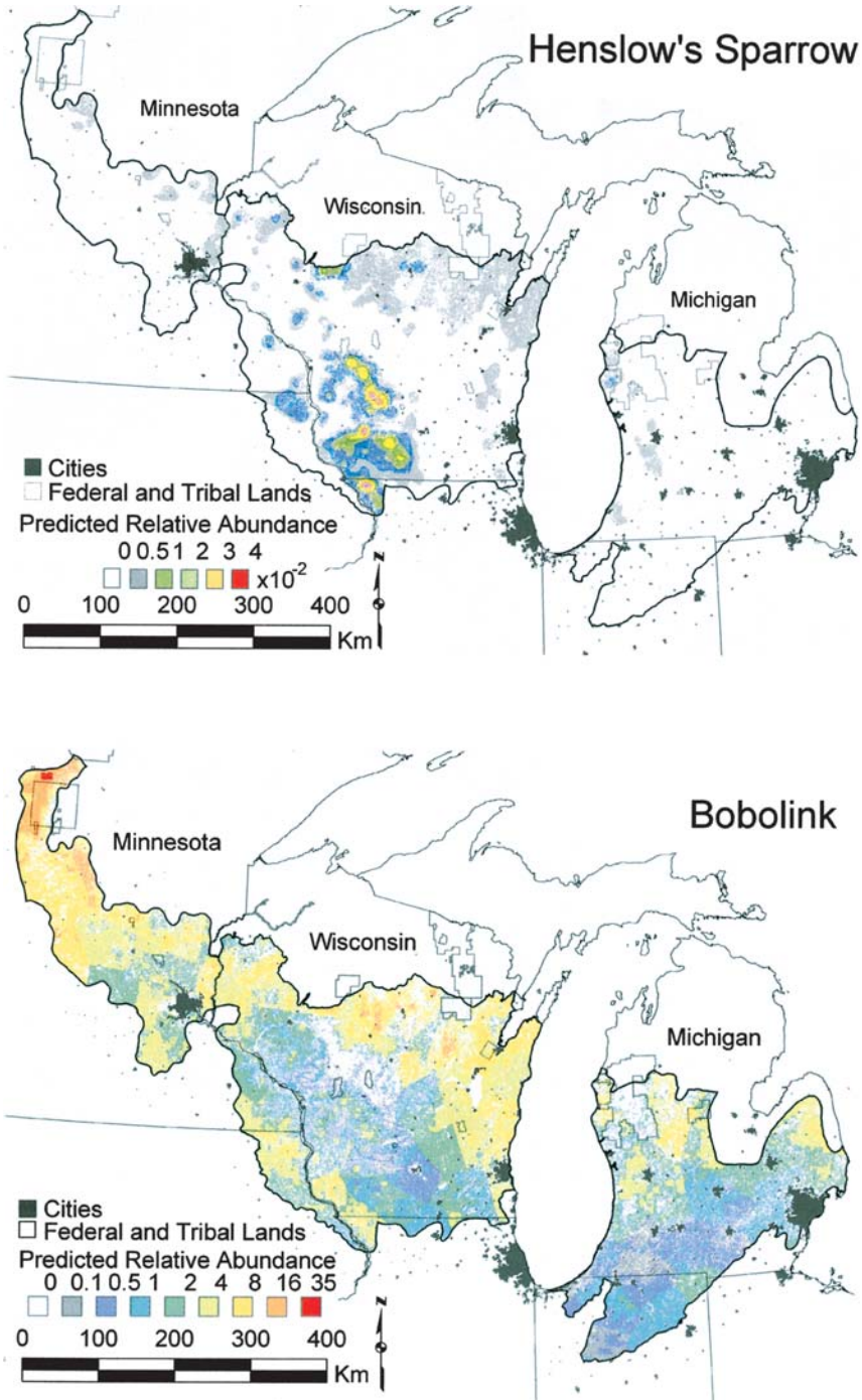
FIGURE 1. (Continued.) Transition of the upper midwestern United States. Note the different abundance scales for each species.
