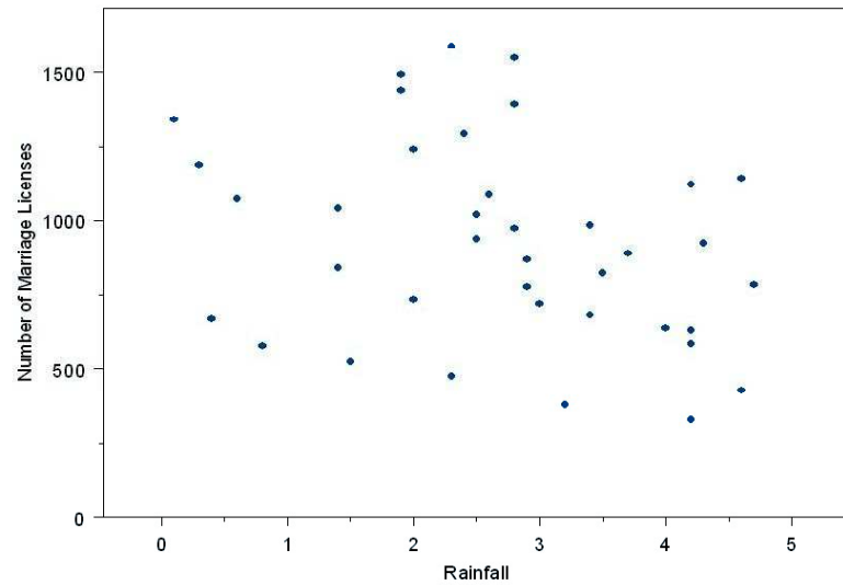
Scatter Plot 3
