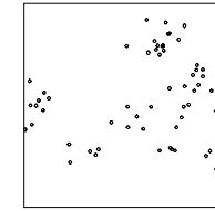
Clustered Pattern
