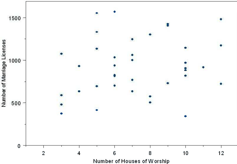
Scatter Plot 1
