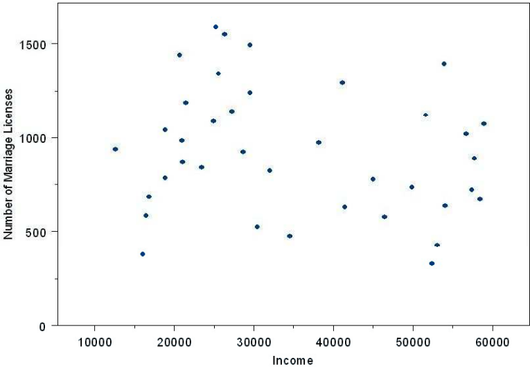
Scatter Plot 2
