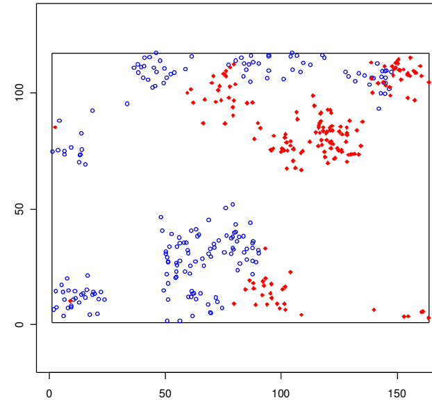
Separate clusters of each type
