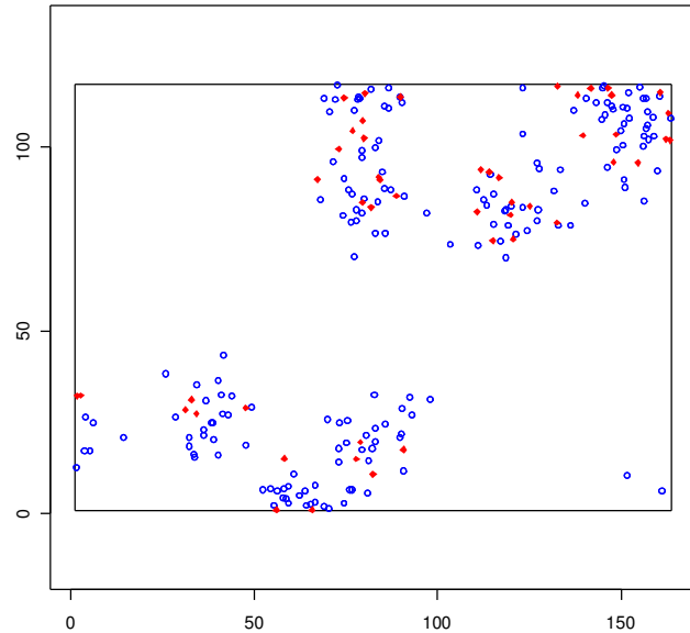
Clusters of diseased trees
