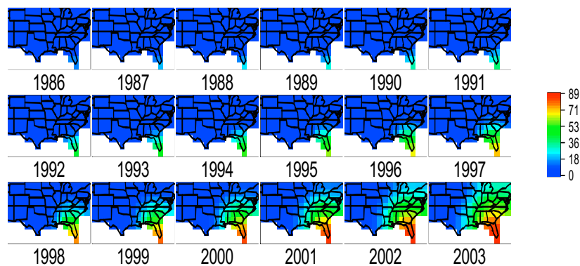
Posterior means for \mathbf{N}
