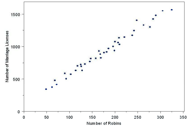
Scatter Plot 4
