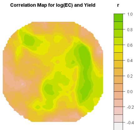
range of r at each point = 100 meters
