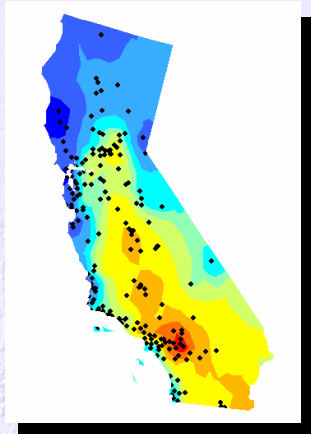
Ozone Predictions
