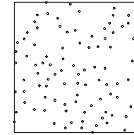
Regular Spacing
