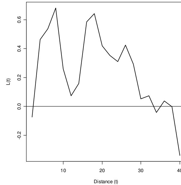
L(t) for all diseased trees
