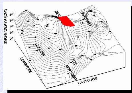
Average Snow Depth
