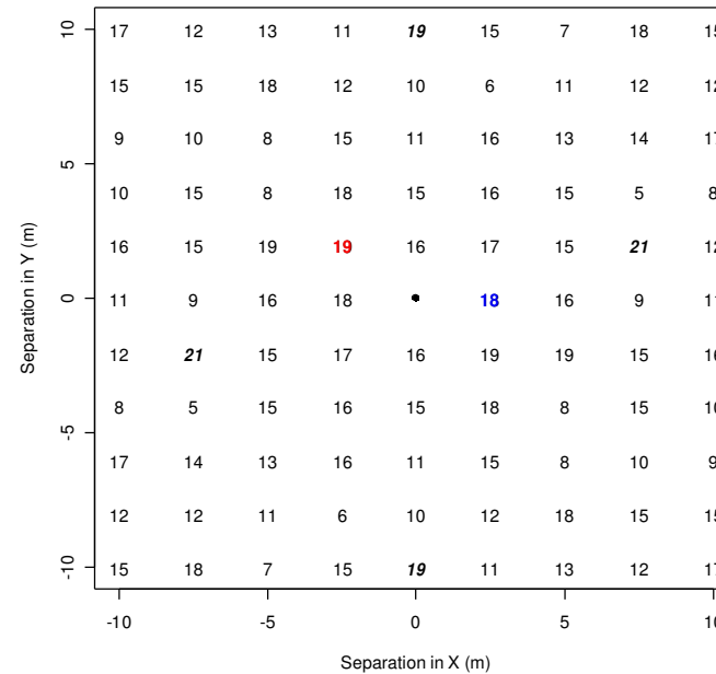
Pairs of diseased trees separated by (x,y)
