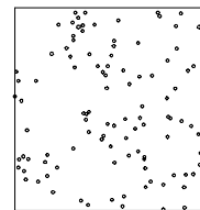
Complete Spatial Randomness
