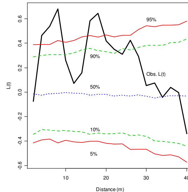
Comparing L(t) to point-based simulation
