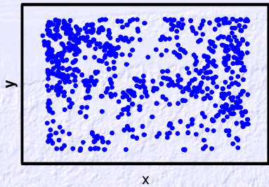
Lansing Woods Hickory Locations
