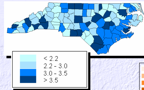
Transformed SIDS rates
