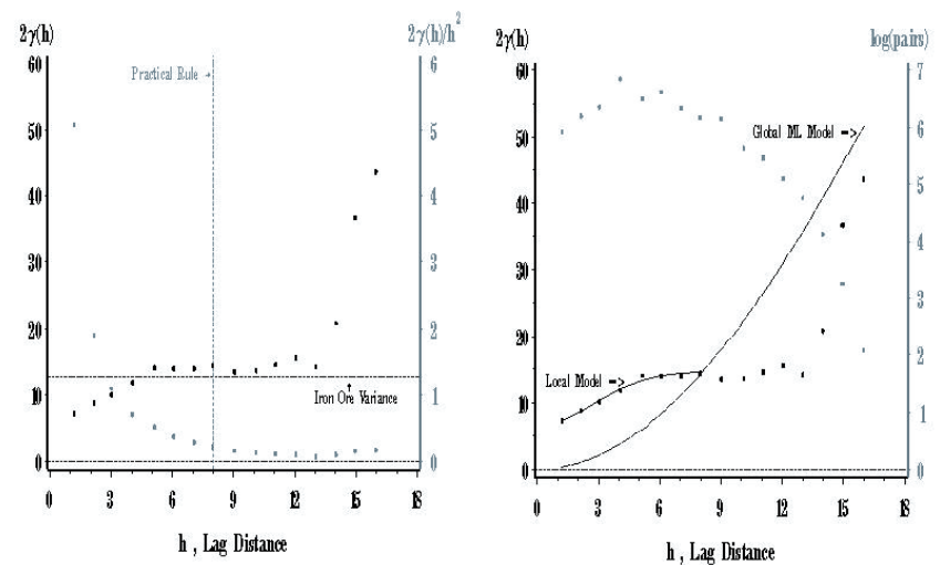
A. Variogram and Regularity Test
