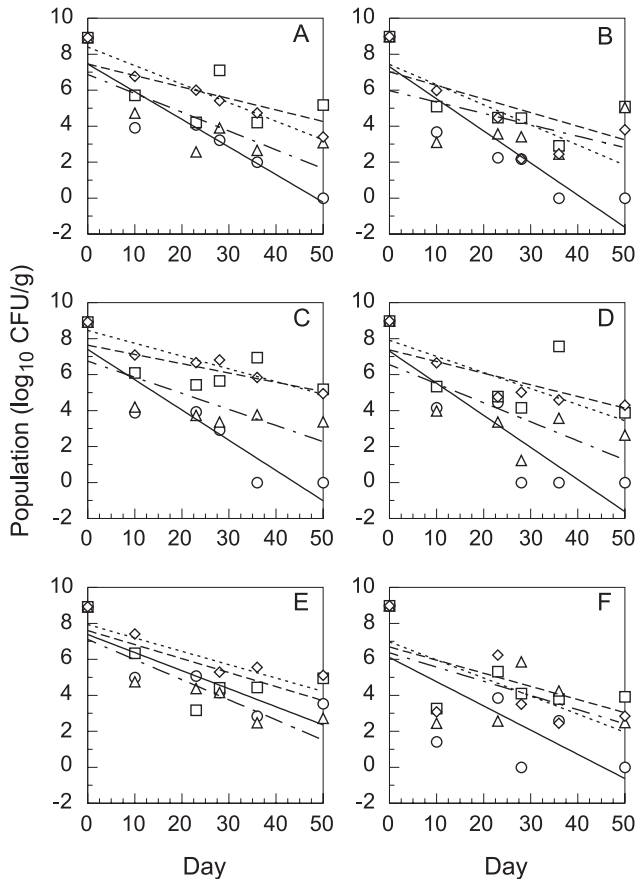
Fig. 2. Linear regression curves showing predictive models for persistence of Escherichia coli O157:H7 in sand and clay soils. The following regression lines represent data from plate count (○); real-time polymerase chain reaction with stx1 (□), stx2 (△), and eae (◇) genes. Pesticide concentrations were at the normal agricultural application rate for (A) methyl bromide (MeBr) sandy soil, (B) MeBr clay soil, (C) methyl iodide (MeI) sandy soil, (D) MeI clay soil, (E) nonfumigated sandy soil, and (F) nonfumigated clay soil. All regression models (see Table 1) used log transformed data.
