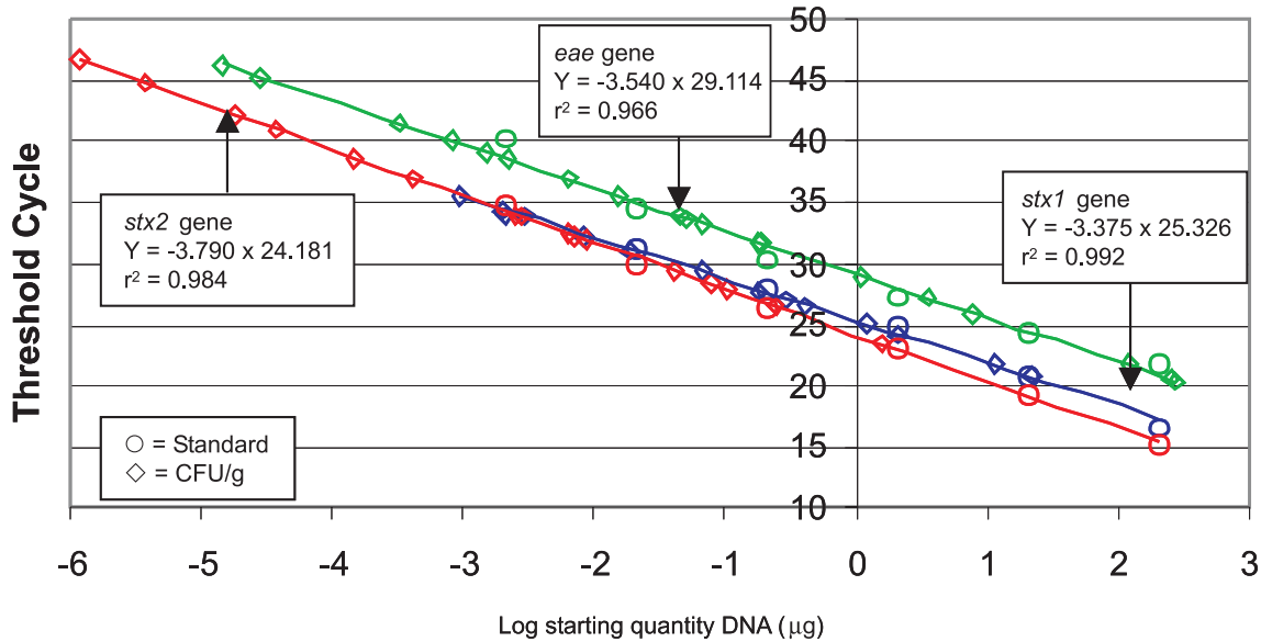
Fig. 1. Standard curves from multiplex real-time polymerase chain reaction analysis of Escherichia coli O157:H7 in microcosm soil showing threshold cycle ( C_T ) versus log DNA starting quantity. The curve (as an example) was used to generate detection limits for quantification of E. coli O157:H7. The reaction efficiency for the stx1 and stx2 genes were better than that of eae gene, as seen by the closeness of the standard curves and with r^2 greater than 0.96. C_T values of known (standard) quantities ( \circ ) and unknown ( \diamond ) samples were plotted against corresponding DNA starting quantities.
