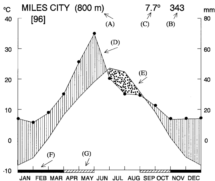
Figure 1. Climate diagram developed for Miles City, Montana, using data from a 96-year period (1900–1996). Included are (A) elevation, (B) mean annual precipitation (mm), (C) mean annual temperature (°C), (D) mean monthly precipitation (mm), (E) mean monthly temperature (°C), (F) average monthly minimum temperature less than 0°C, and (G) absolute monthly minimum temperature less than 0°C. Data for the area indicate mesic spring, early summer, and autumn periods interrupted by late summer and early autumn drought (stippling). Winter precipitation occurs as snow. Figure follows standard form of Walter (1985).
